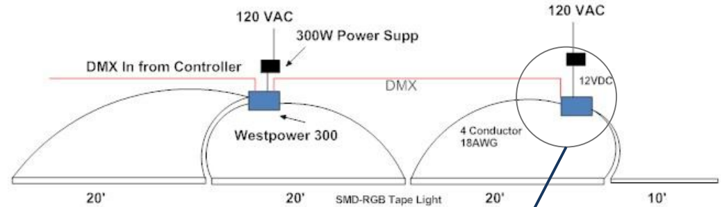
SMD RGB Tape and Westpower Layout
