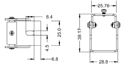
Dimensions Unit: mm
