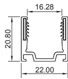
Dimensions Unit: mm
