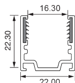
Dimensions Unit: mm
