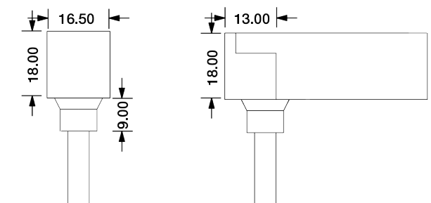
Bottom Entry Connector TPR-KFLDV-PC-BC
