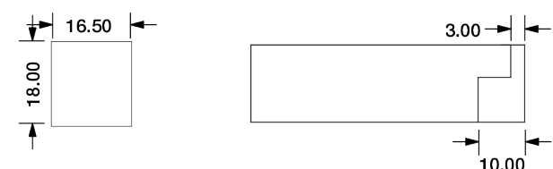
End Cap TPR-KFLDV-PC-ECAP
