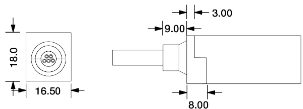
Direct Entry Connector TPR-KFLDV-PC-EC
